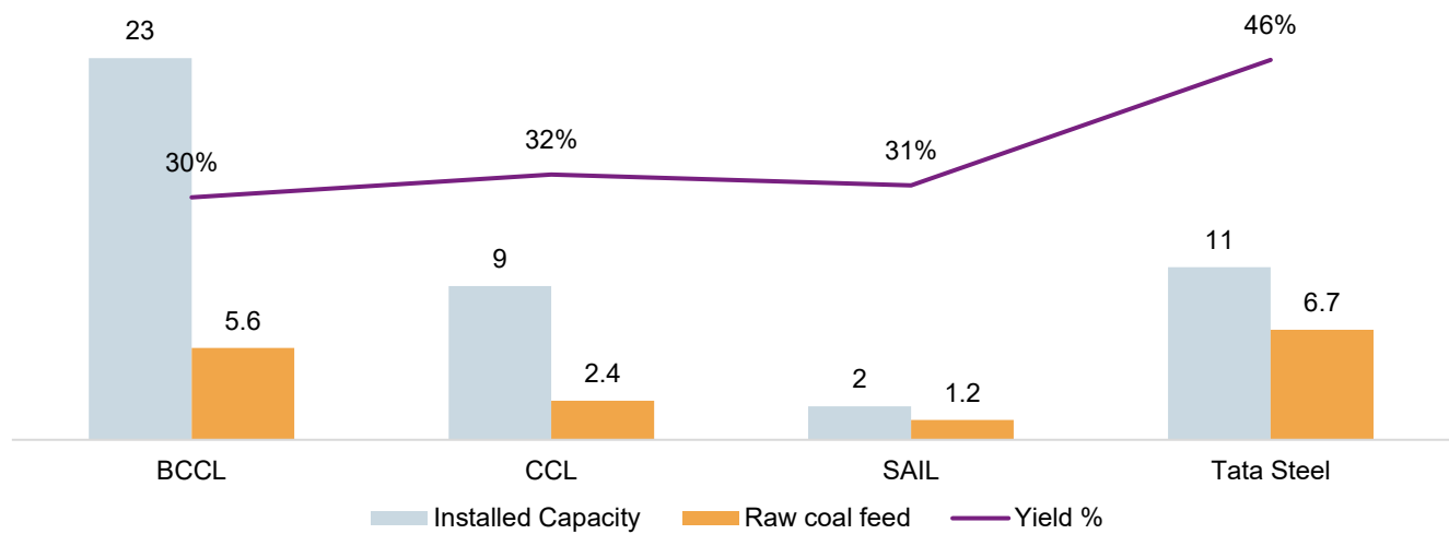
Figure 3.40 Coking coal washery performance in fiscal 2025 (MMT)
